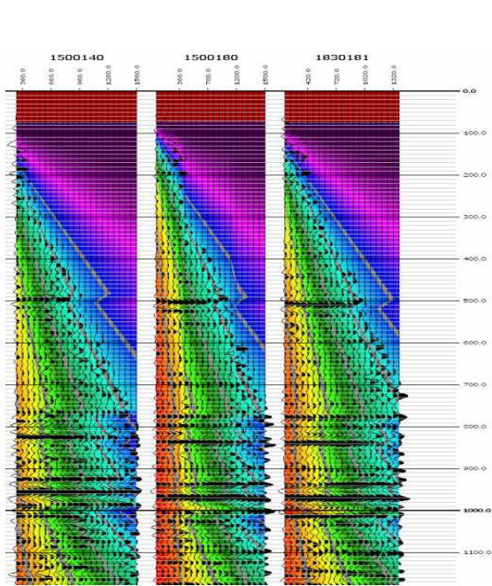
Overlay of angle information on offset
