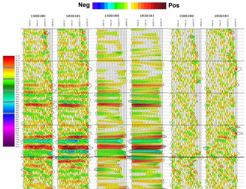
Input gathers Reconstructed gathers Difference
