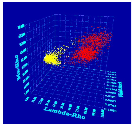
3D Cross-plotting of Lambda-Rho, Mu-Rho and Fluid Stack. Clusters associated with gas anomalies (yellow) separate out.
